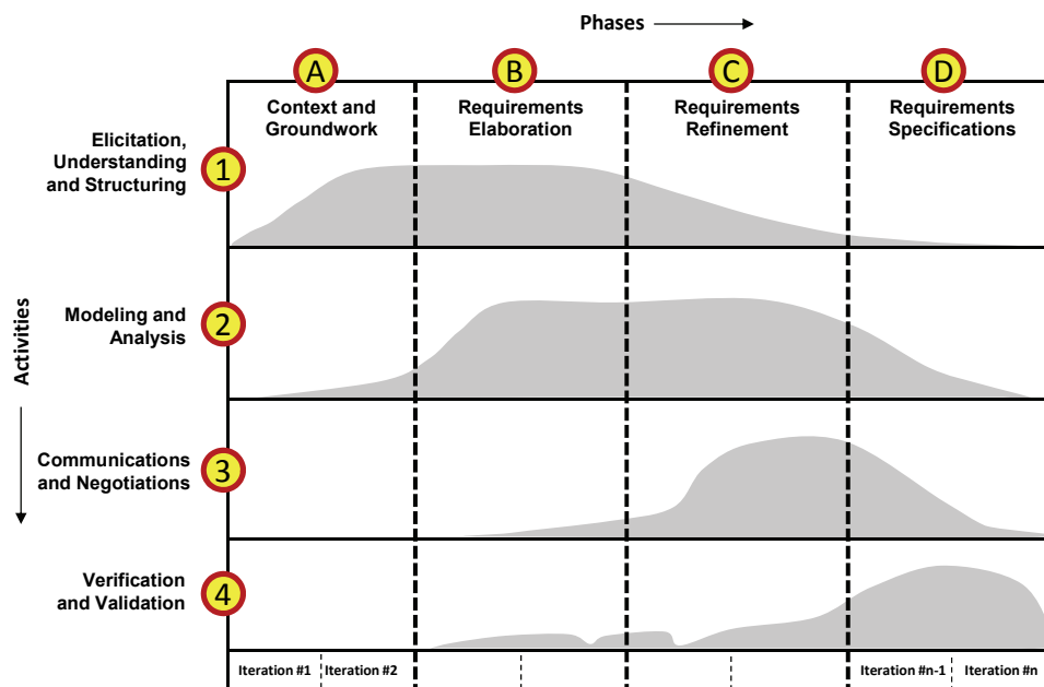
Figure 1: Requirements Engineering Lifecycle – A Unified Perspective of the RE Process [30]
